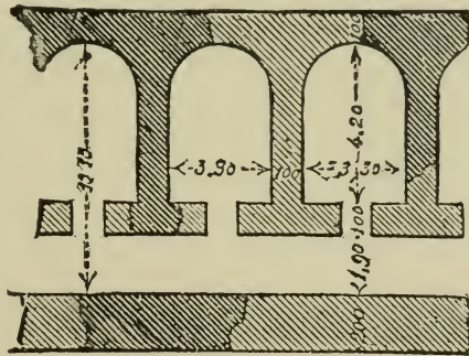
PLAN OF WALL AT BYRSA.
